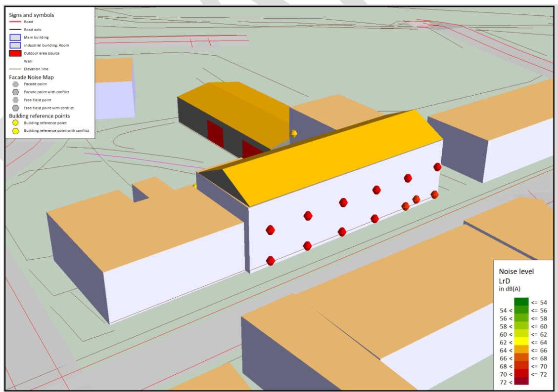
Figure 4 – Daytime FNM of both traffic and industrial noise, Church Street West (front)
