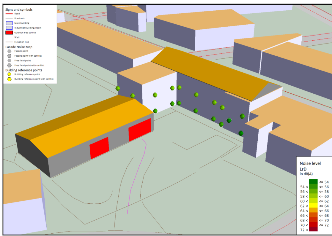
Figure 5 – Daytime FNM of both traffic and industrial noise, Church Street West (rear)
