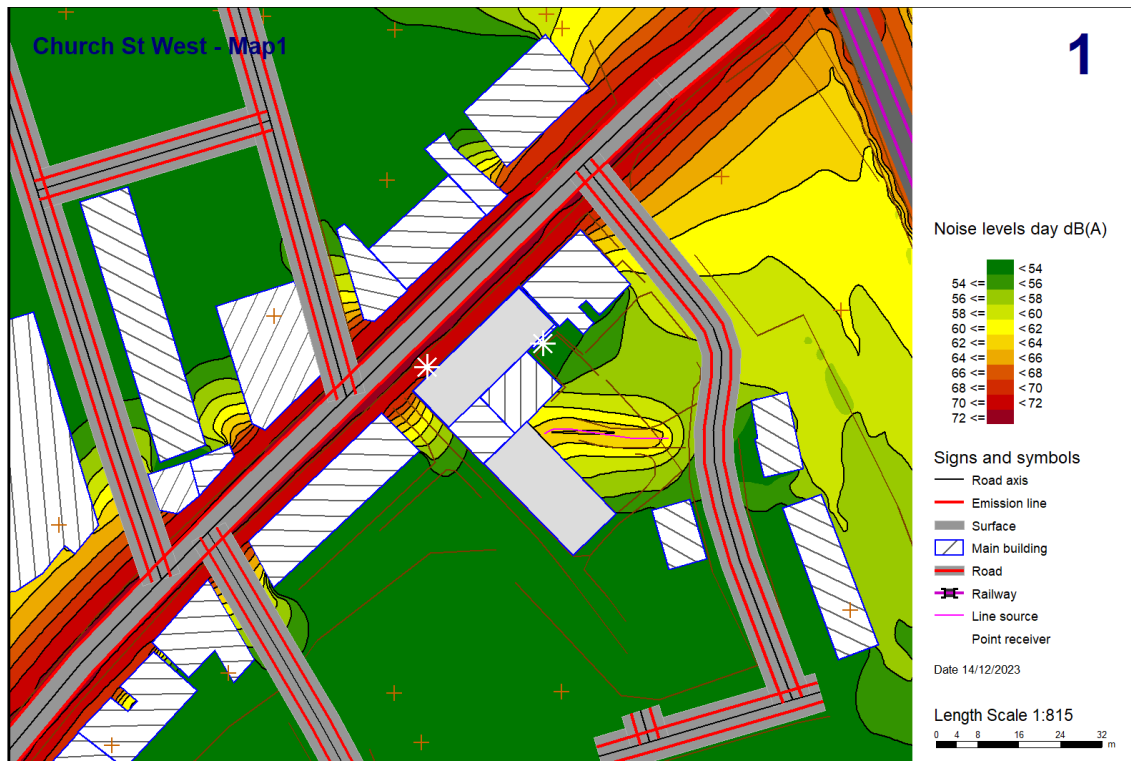
Figure 3 – Daytime GNM of both traffic and industrial noise, Church Street West
