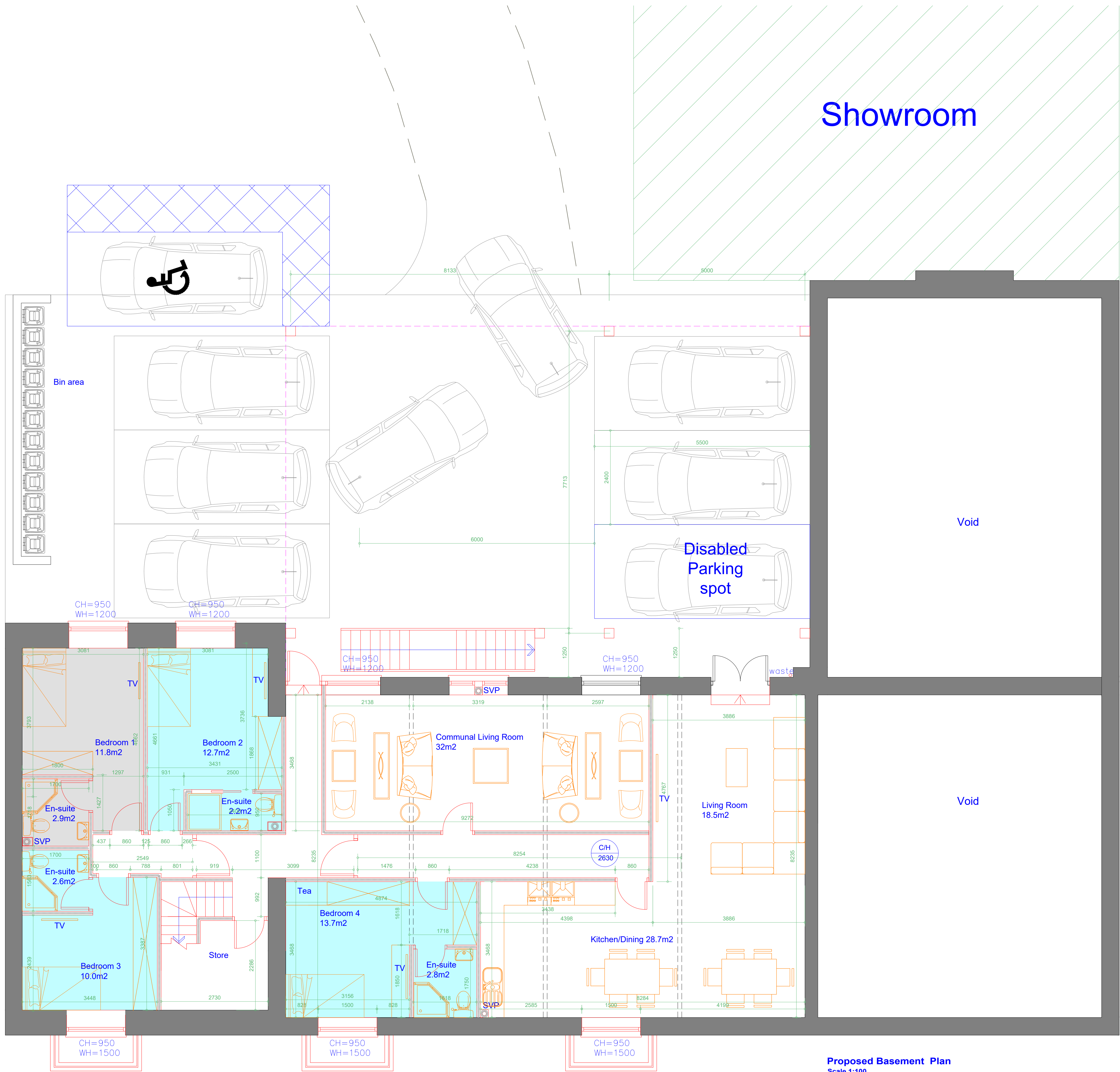
Proposed Basement Plan Scale 1:100
