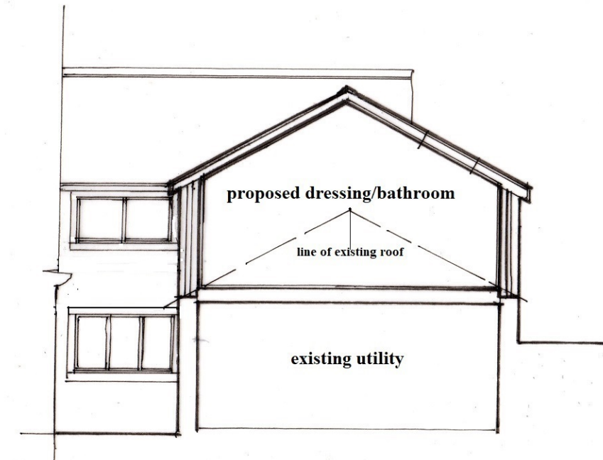
Proposed Section
