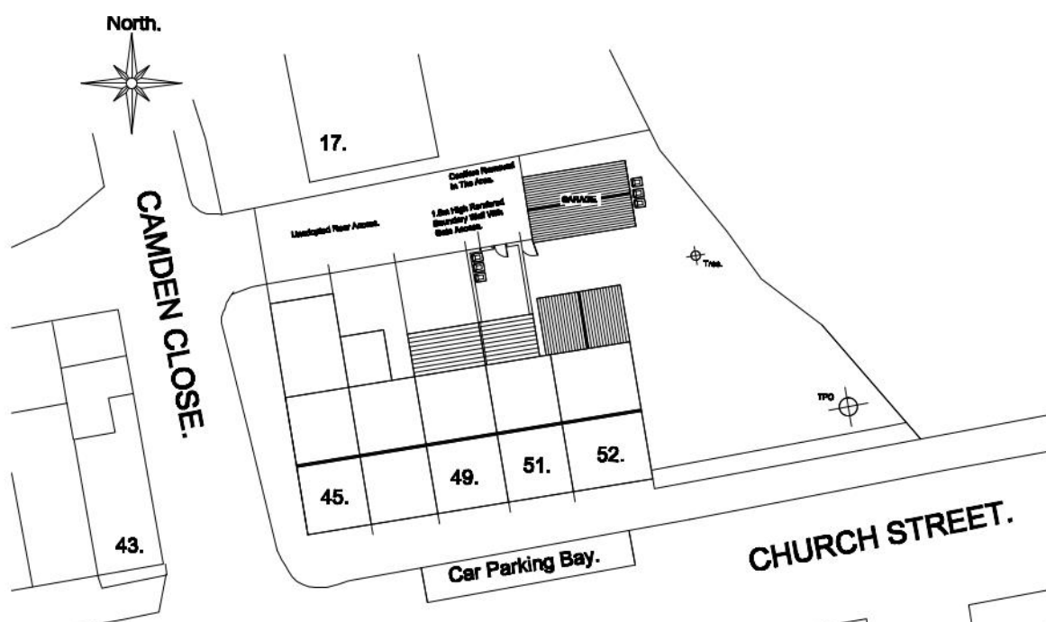
Figure 2 – Site plan for the proposed Church Street residential development.
