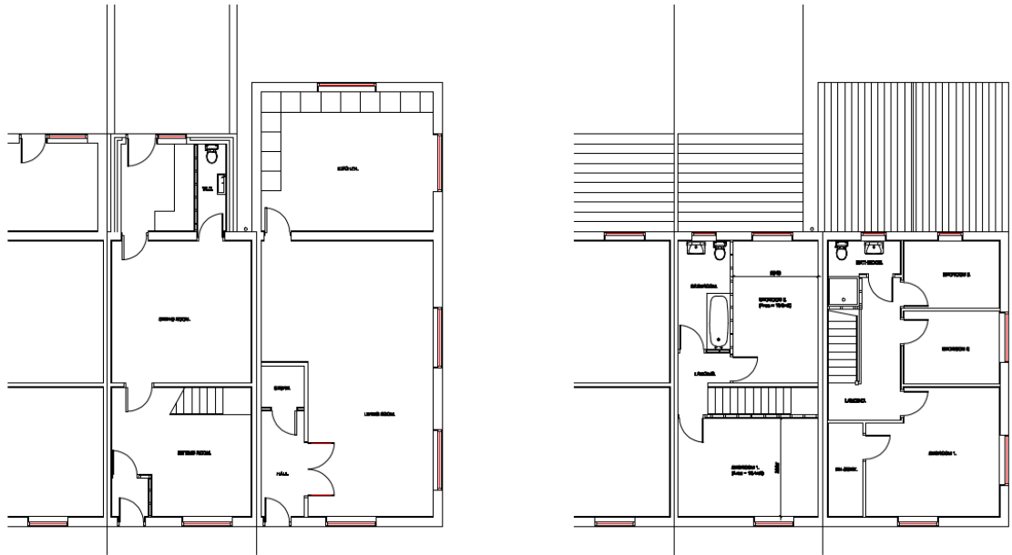
Figure 3 – Proposed Dwelling conversion Floor Plans
