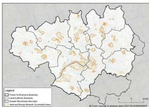
Figure 5.1 Heat and Energy Network Opportunity Areas
