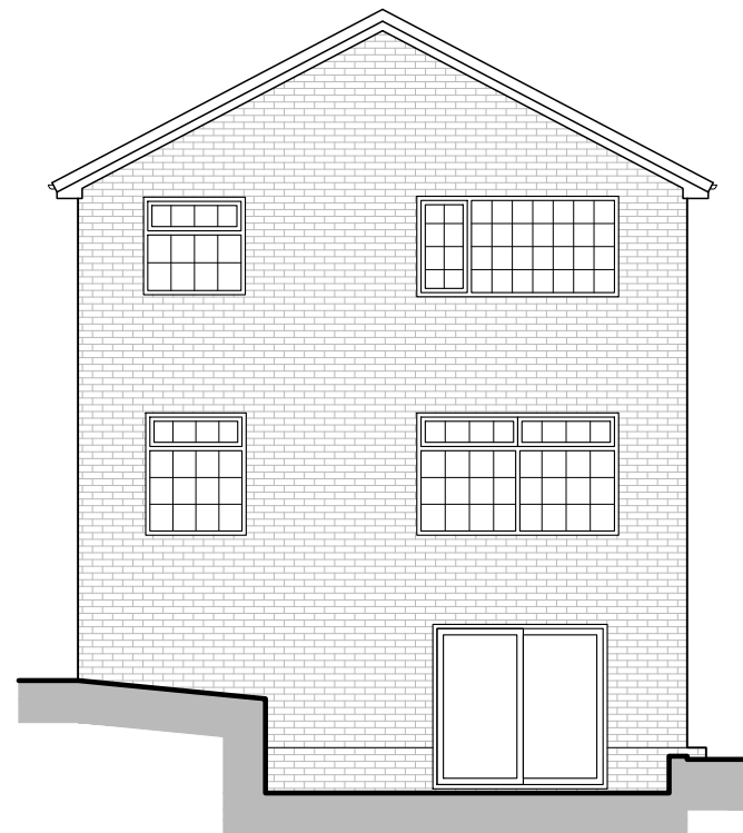
NORTH WEST ELEVATION - 1:100
