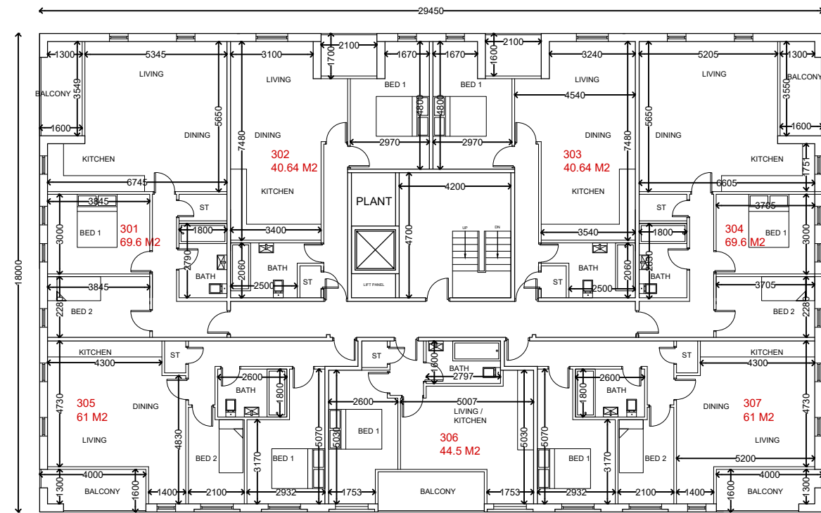
THIRD FLOOR PLAN 7 APARTMENTS - 4 TWO BEDS - 3 ONE BED
