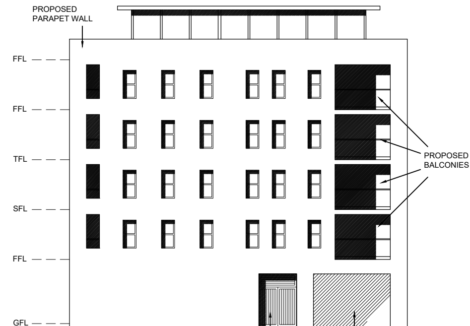
SIDE ELEVATION
