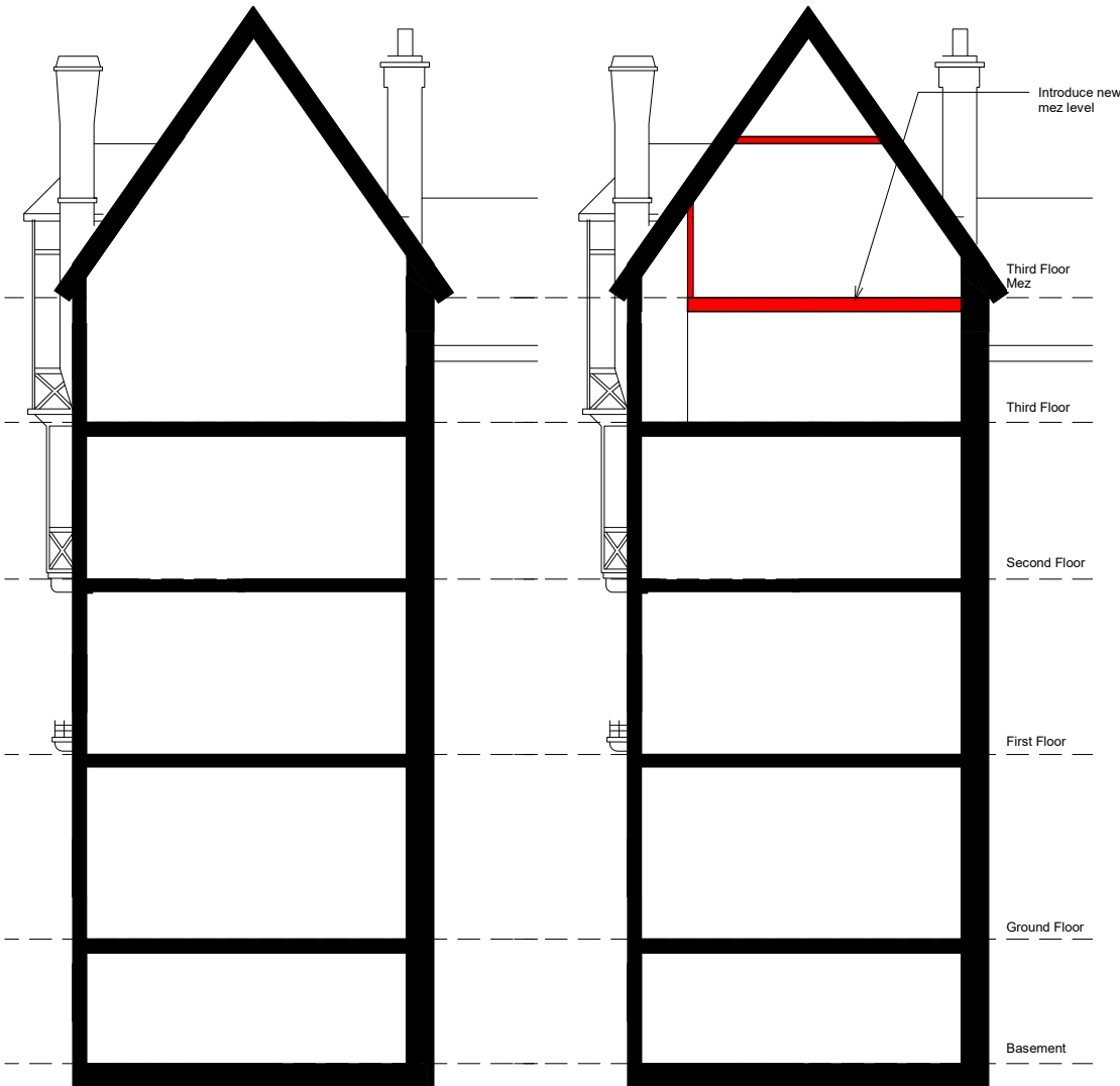
Proposed section showing staircase on Mez level
