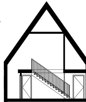
Proposed section showing staircase on Mez level
