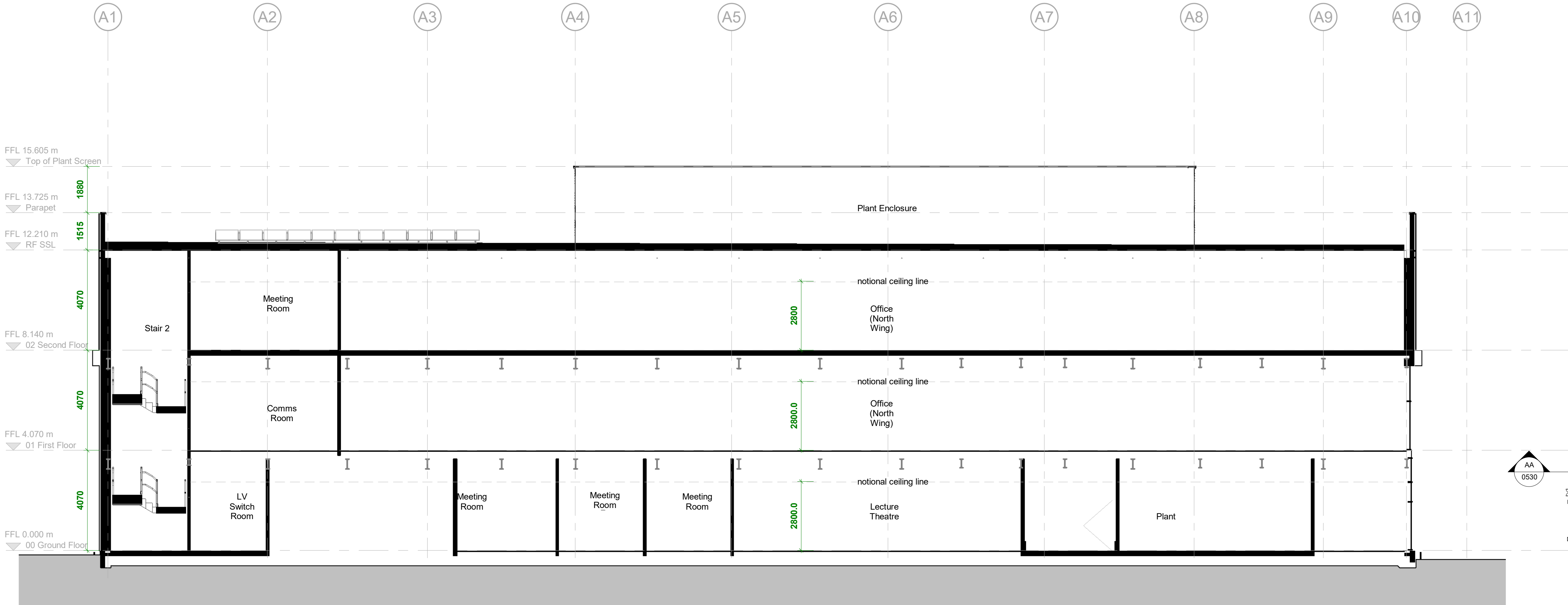
Section AA - Through North Wing
