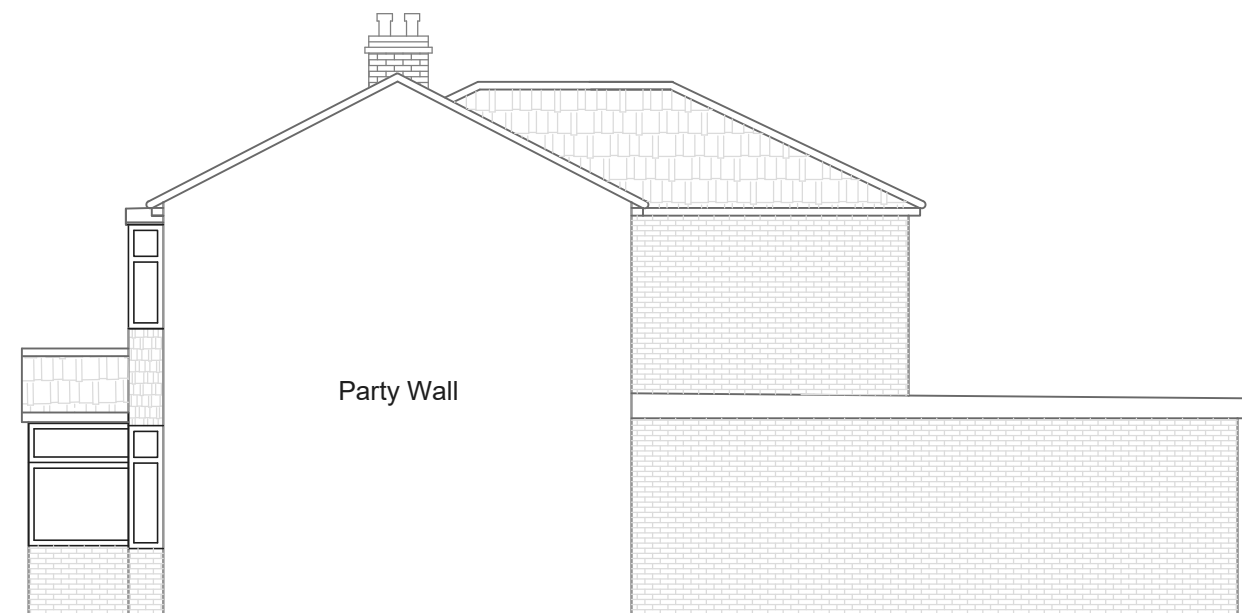
PROPOSED SIDE EXTENSION (EAST)
