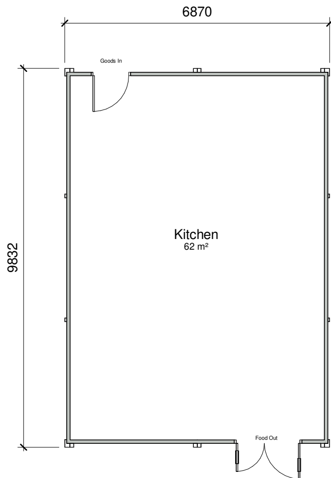
1 Ground Floor 1 : 100
