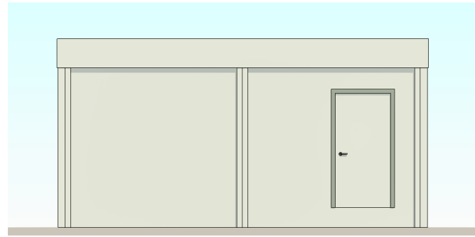
3 West Elevation 1 : 100
