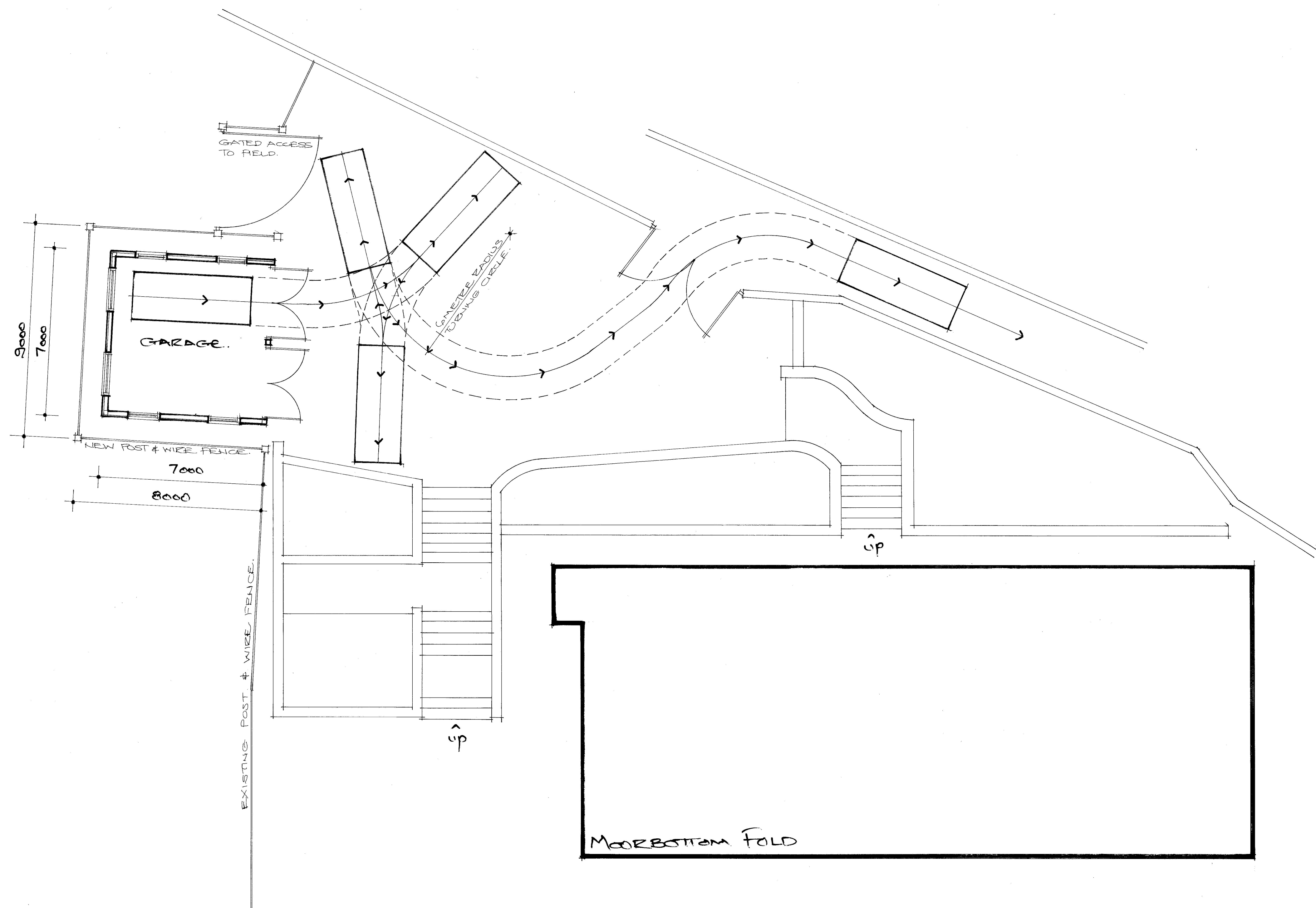
PROPOSED GARAGE LAYOUT
