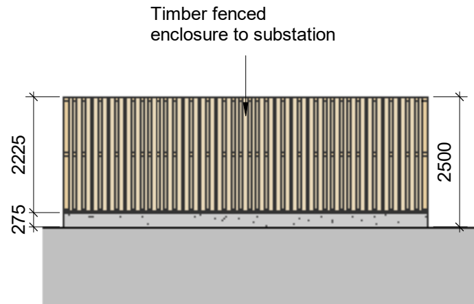
4 Proposed South East Elevation Scale @ 1 : 100
