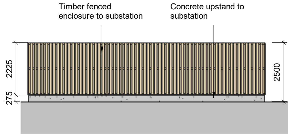
3 Proposed South West Elevation Scale @ 1 : 100
