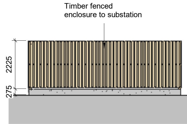
2 Proposed North West Elevation Scale @ 1 : 100
