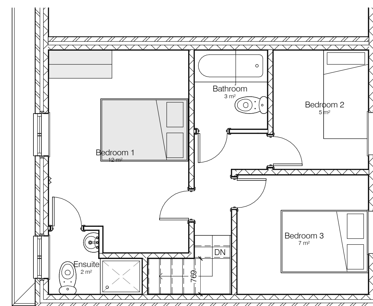
Existing First Floor Plan 1 : 50
