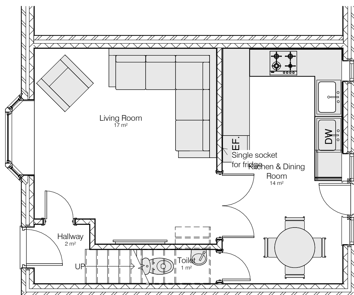
Existing Ground Floor Plan 1 : 50
