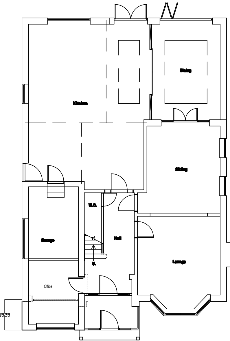
PROPOSED GRD. FLOOR PLAN
