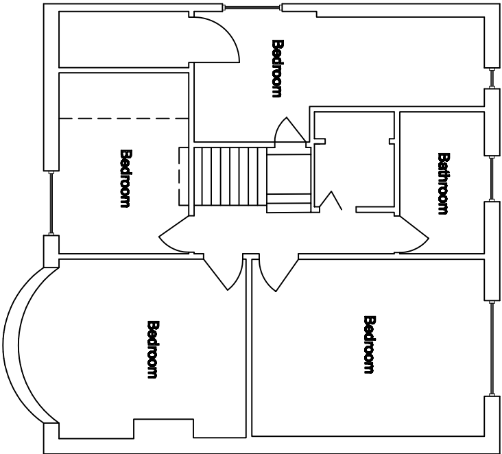
First Floor
