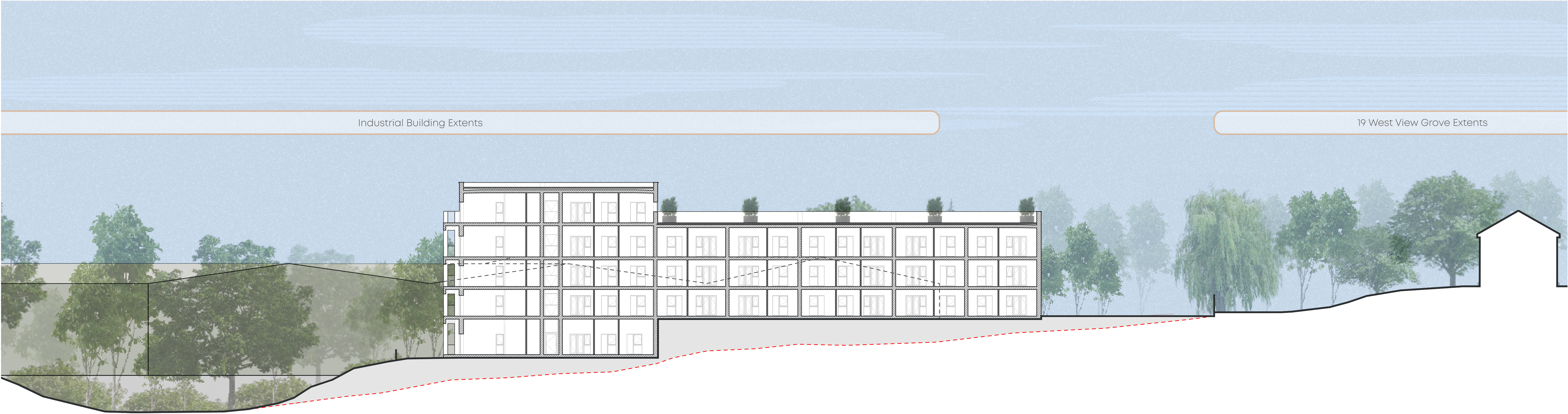
Section A-A Proposed Scale: 1:200
