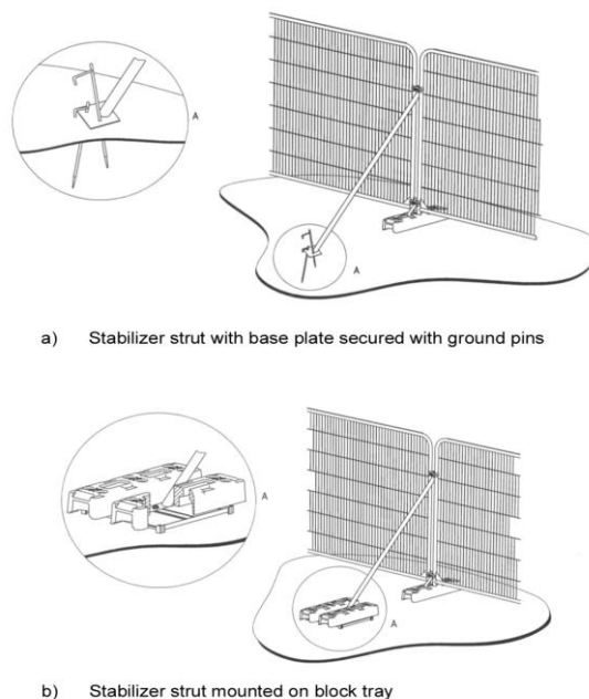
Fig 1. Tree protection fencing specification (extract from BS 5837: 2012)
