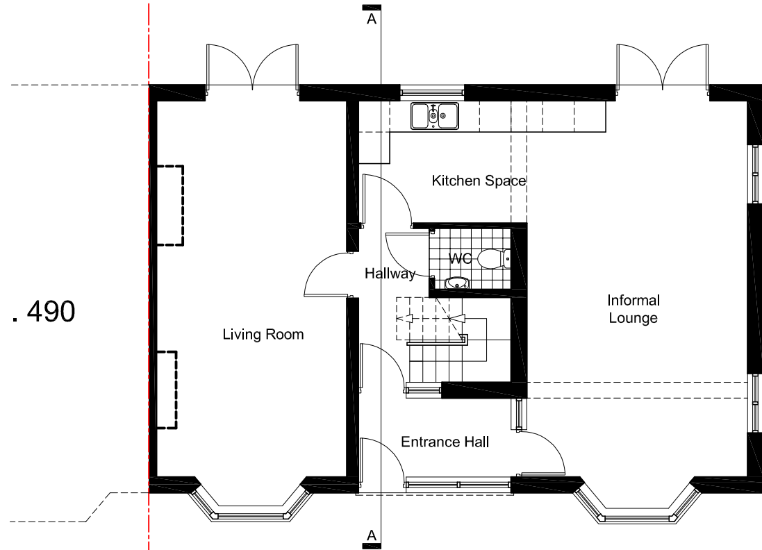
Proposed GF Plan 1:100
