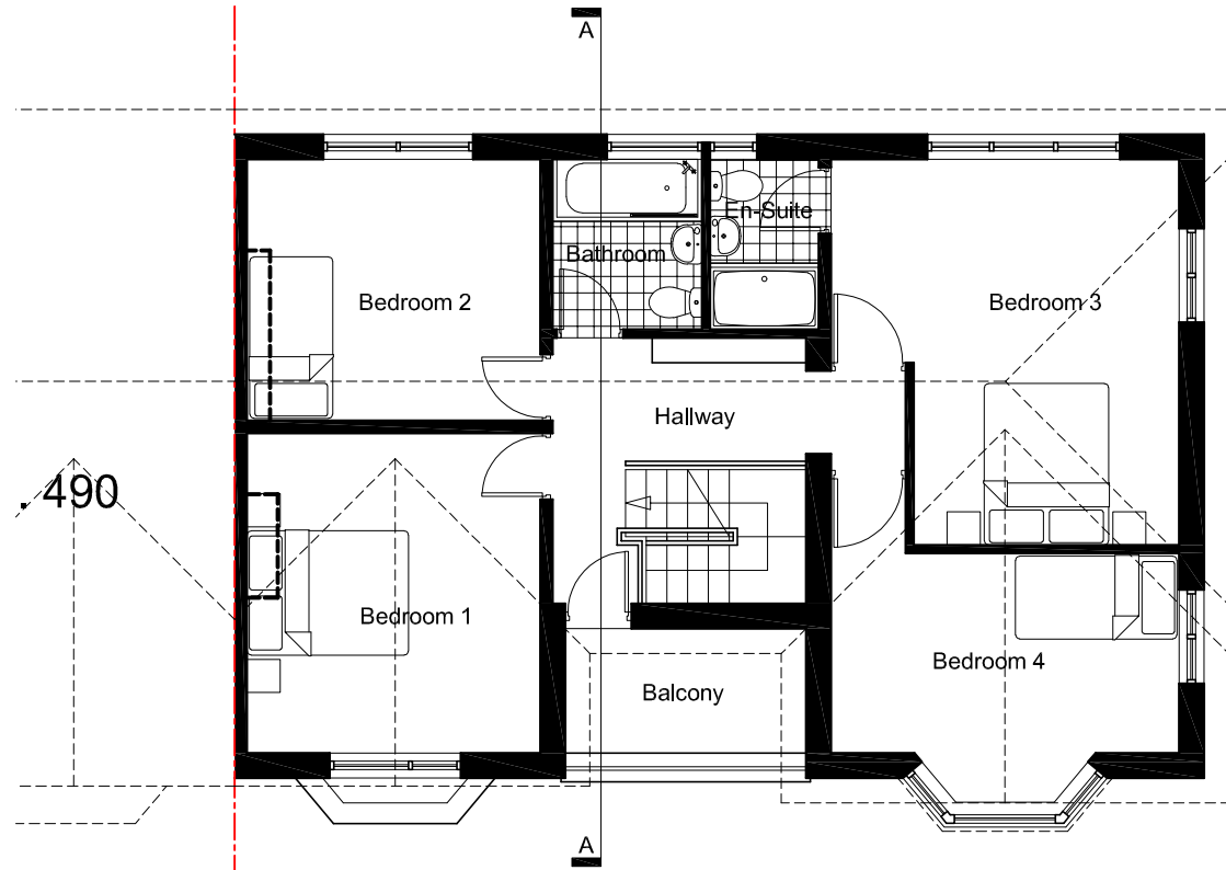
Proposed 1F Plan 1:100
