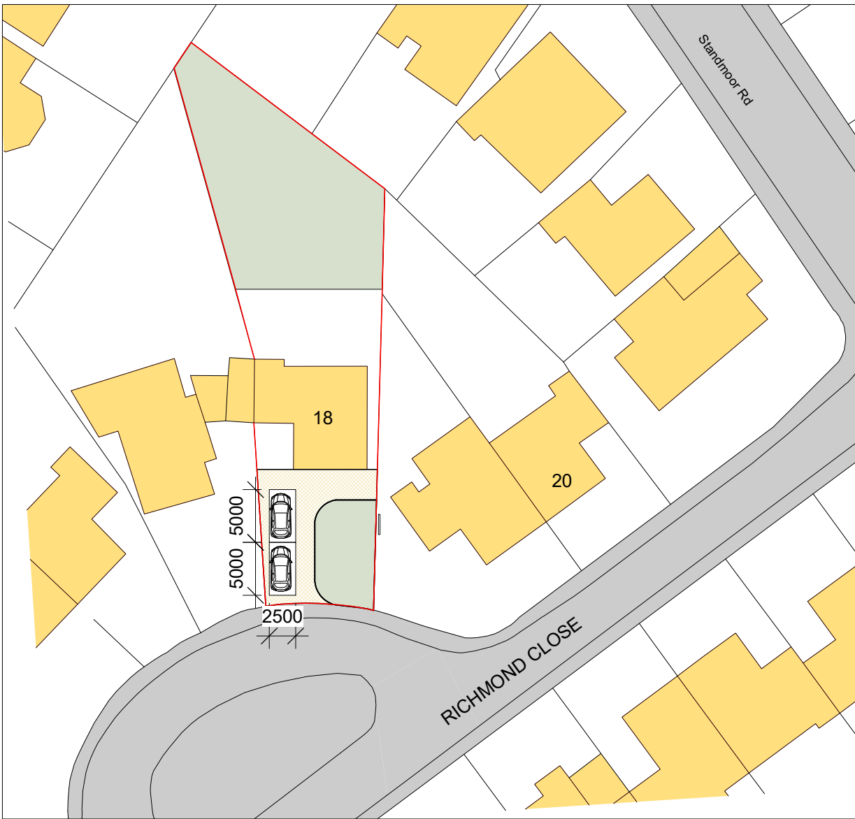
2 Existing Site Layout Plans 1 : 500
