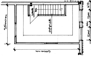
First Floor Plan (Unit 2)
