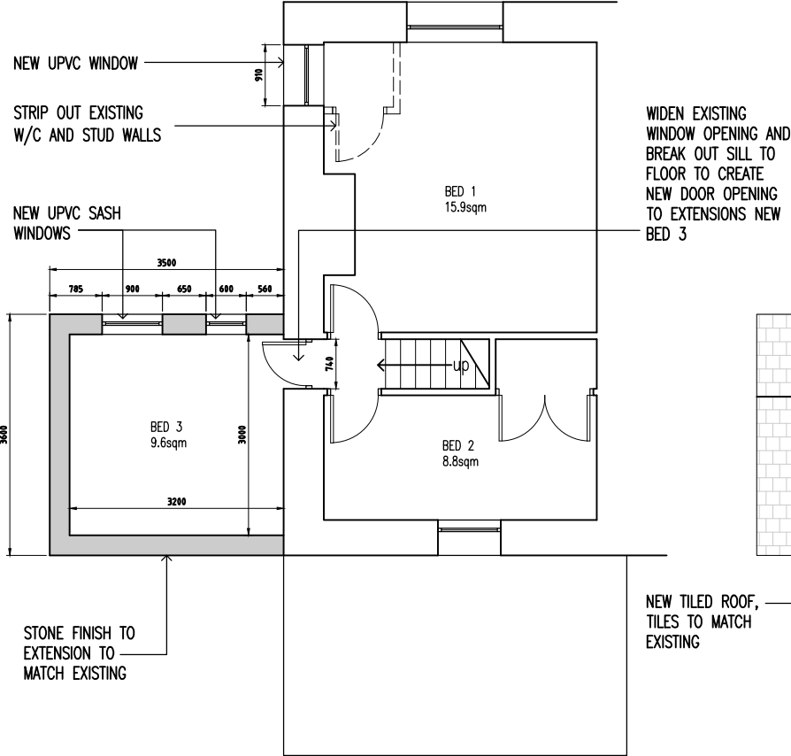
PROPOSED FIRST FLOOR PLAN 1:100 @ A3
