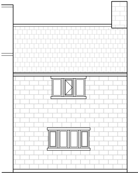
EXISTING FRONT ELEVATION 1:100 @ A3
