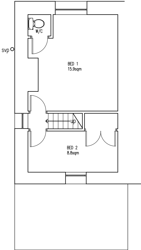
EXISTING FIRST FLOOR PLAN 1:100 @ A3
