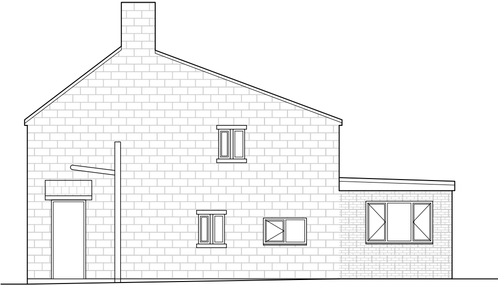
EXISTING SIDE ELEVATION 1:100 @ A3
