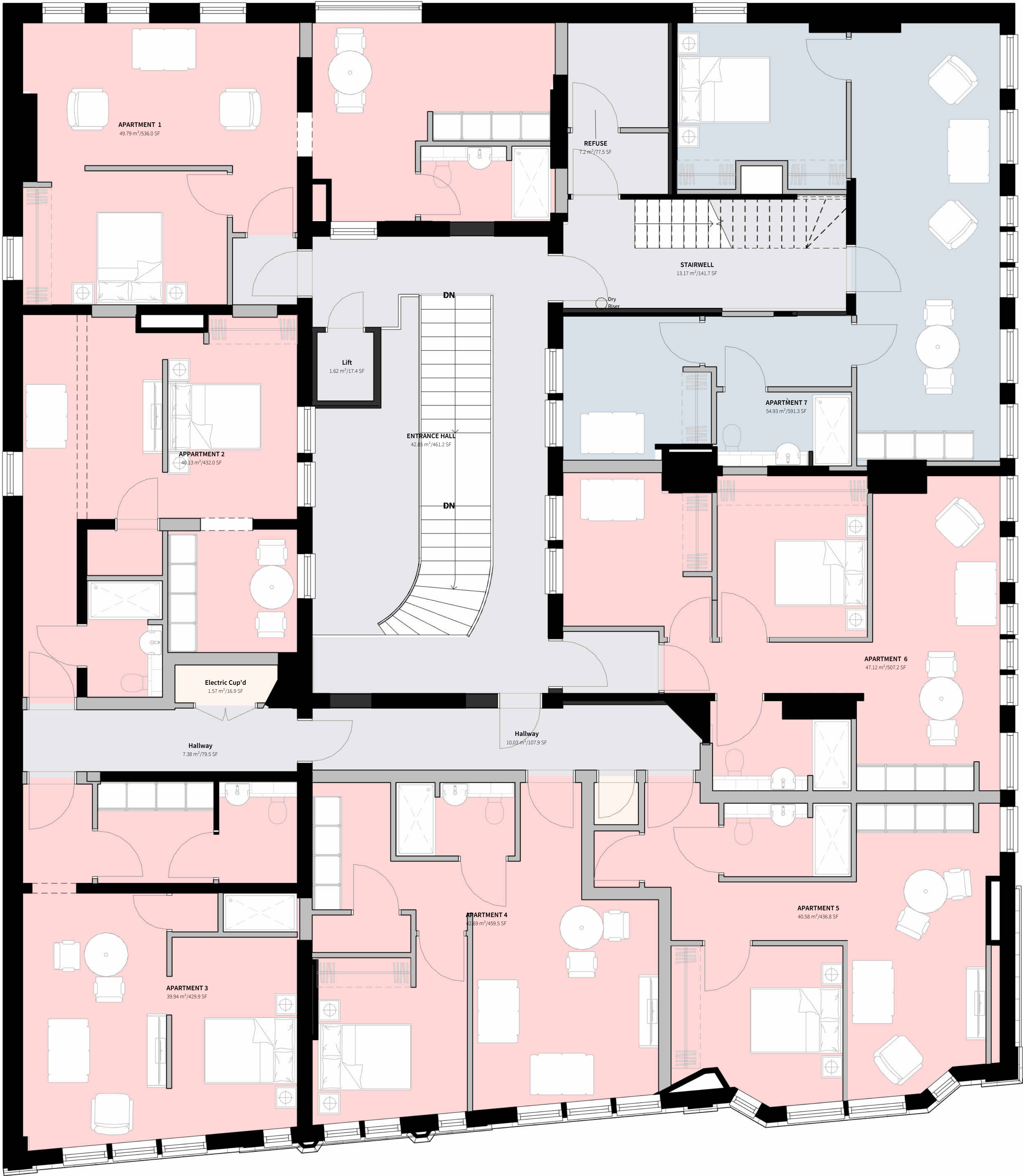
2 Proposed-Plan_01-First 1:50
