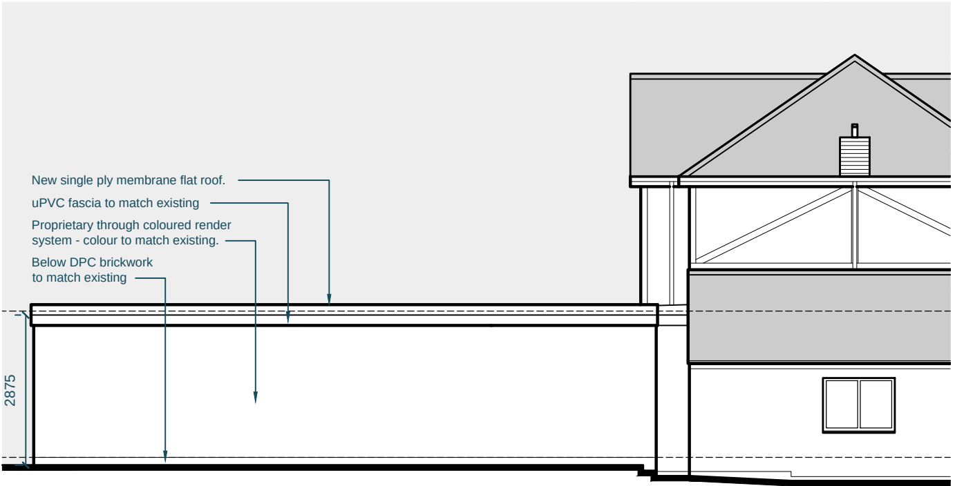
3.West Elevation
