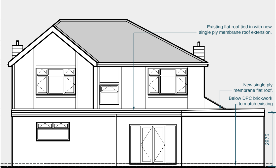
4.South Elevation
