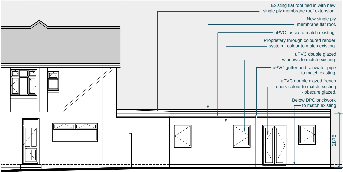
1.East Elevation
