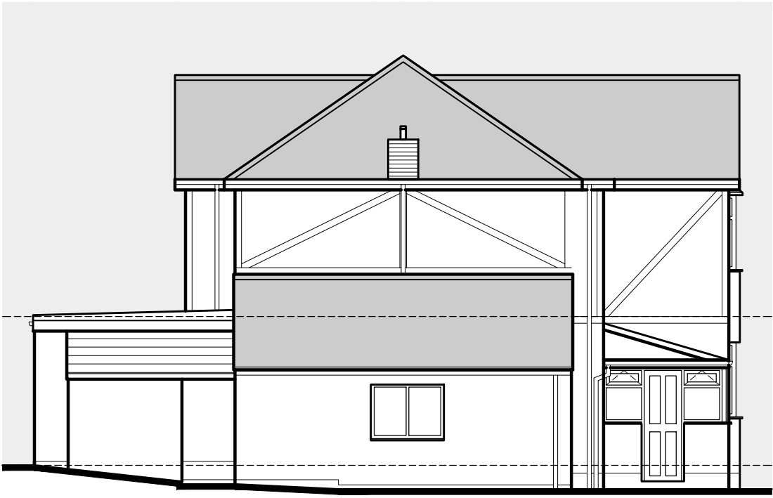
3.West Elevation
