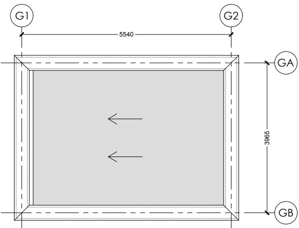
DETACHED GARAGE, PROPOSED ROOF PLAN 1:100
