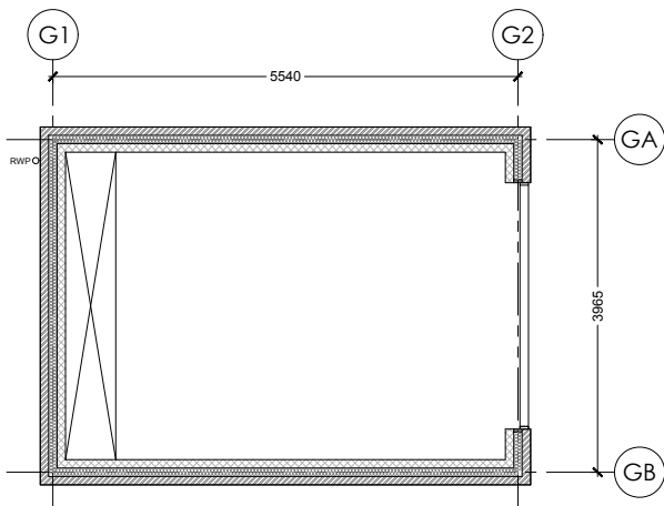
DETACHED GARAGE, PROPOSED PLAN 1:100
