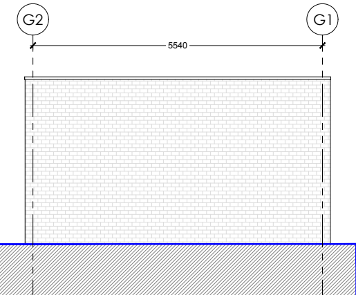
DETACHED GARAGE, SIDE ELEVATION 1:100
