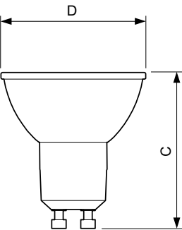
MASTER LED spot VLE DT 4.9-50W GU10 927 36D
