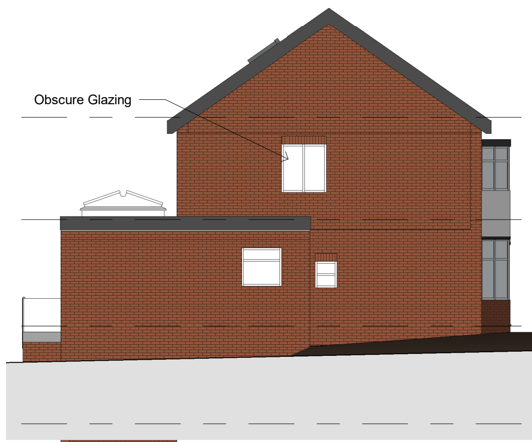
4 Left Side - Proposed 1 : 100
