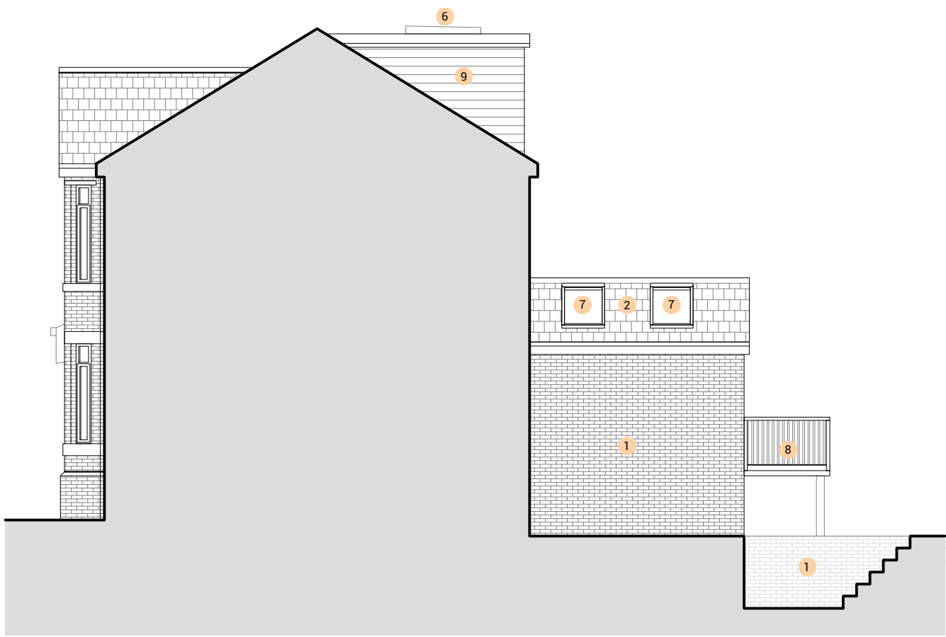
PROPOSED SIDE ELEVATION 1:100 @ A2
