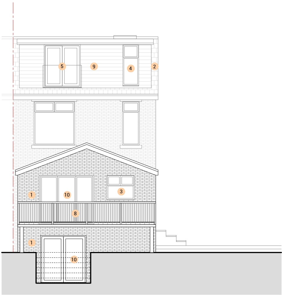
PROPOSED REAR ELEVATION 1:100 @ A2
