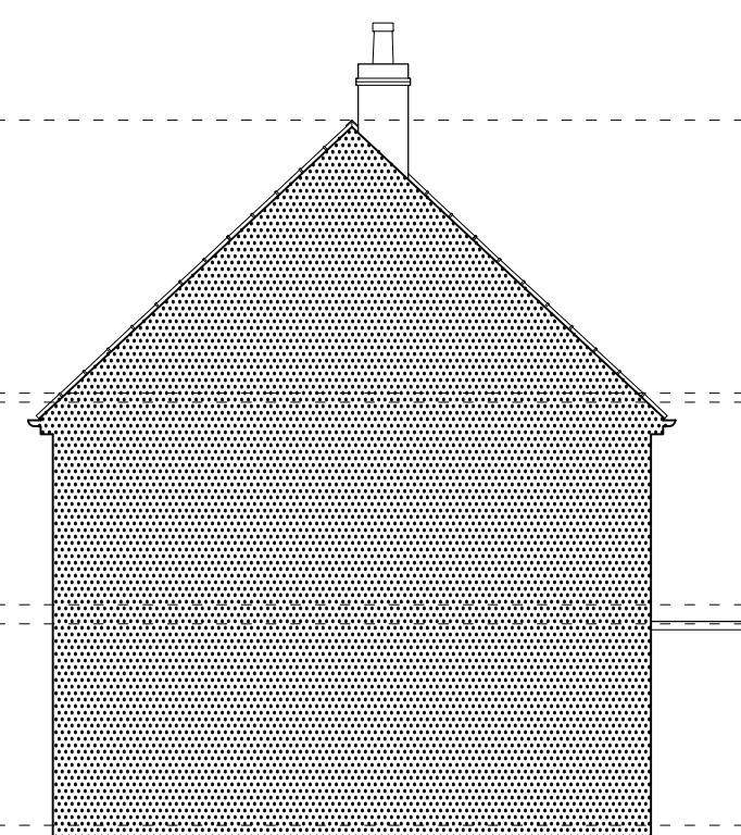
EXISTING SIDE ELEVATION (PARTY WALL)
