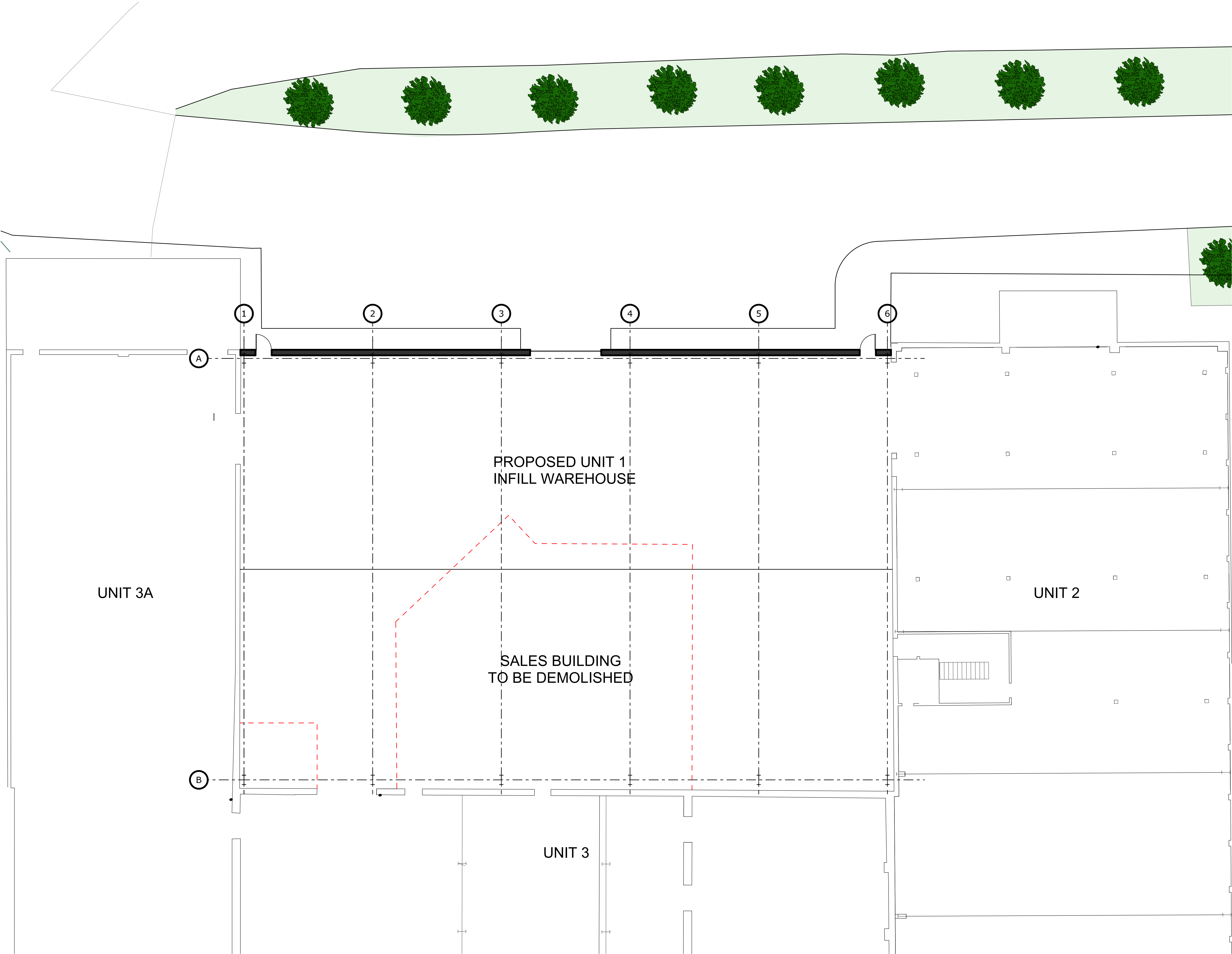
proposed infill warehouse plan 1:100
