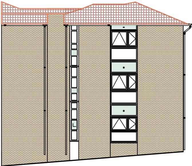
Elevation MP1
