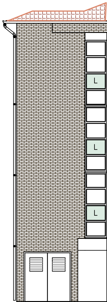
Elevation MP1
