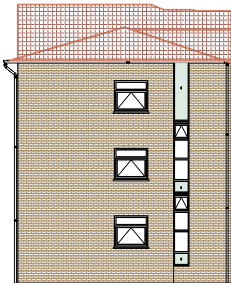
Elevation MP2
