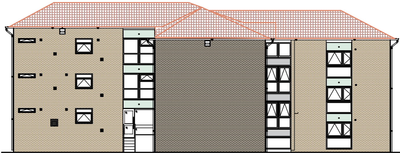
Elevation D
