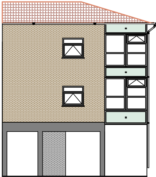
Elevation MP1
