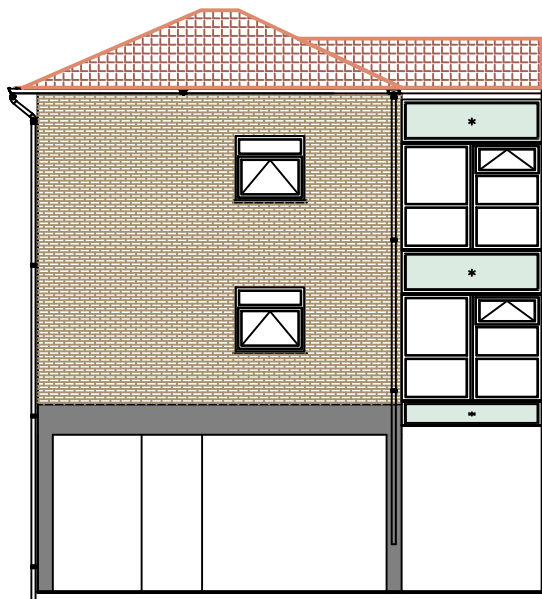
Elevation MP6
