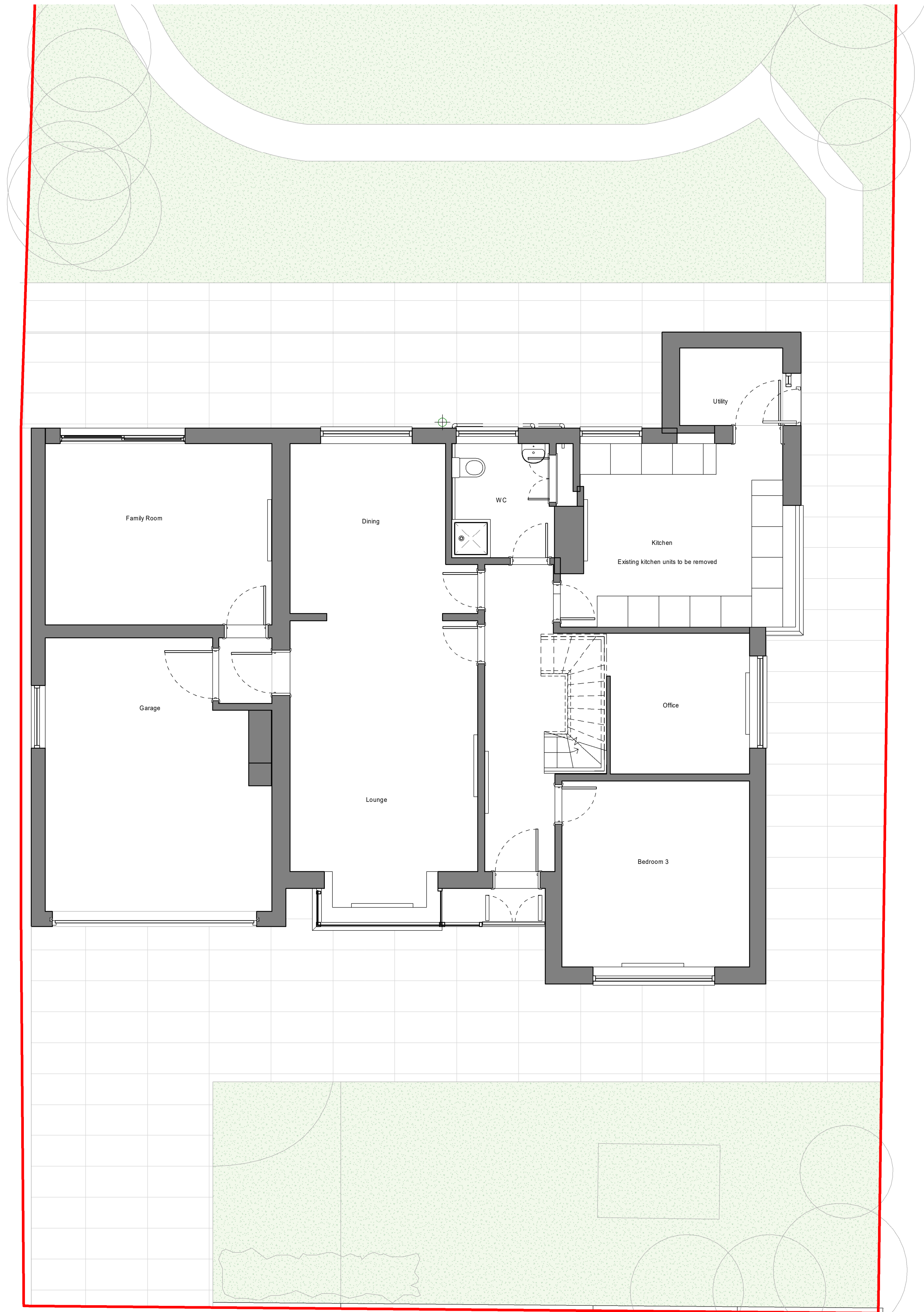
1 Level 0 - Existing GA Plan 1 : 50
