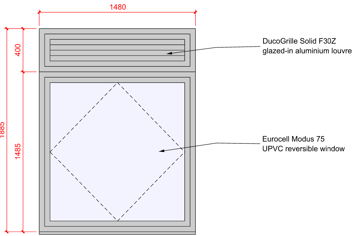
Typical Apartment Window Elevation
