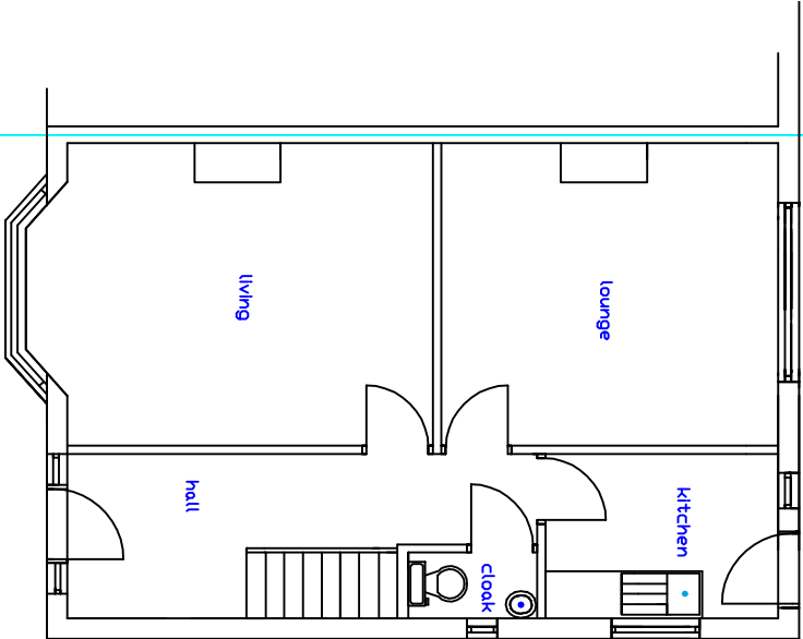
PROPOSED GROUND FLOOR LAYOUT 1:100
