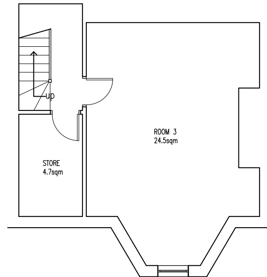
EXISTING BASEMENT FLOOR PLAN 1:100 @ A3
