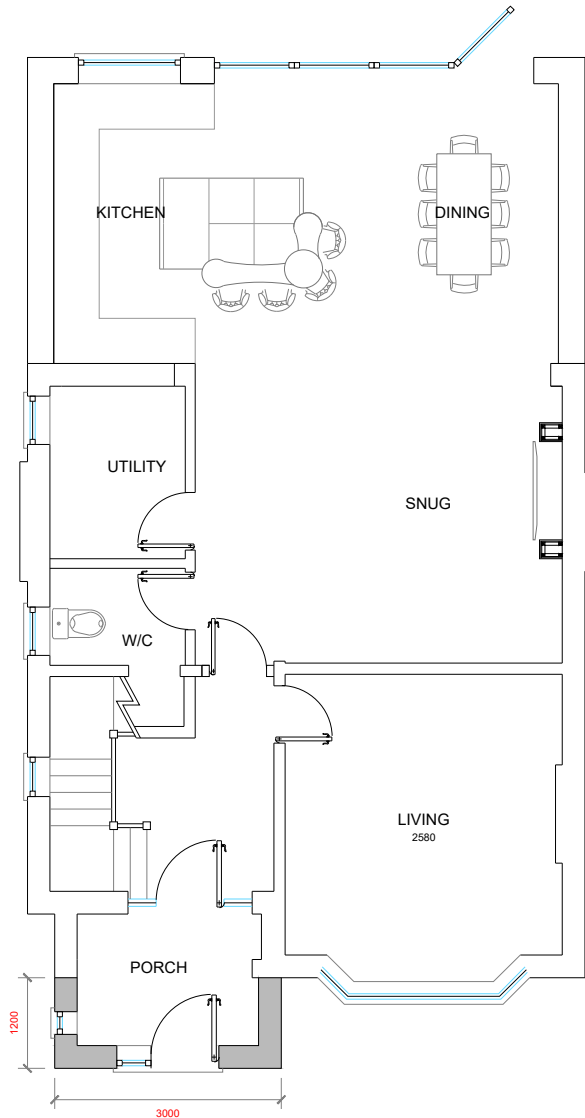
GROUND FLOOR
