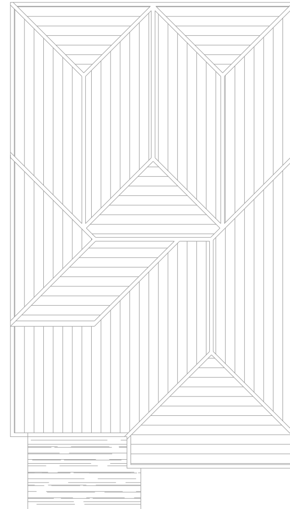
ROOF PLAN
