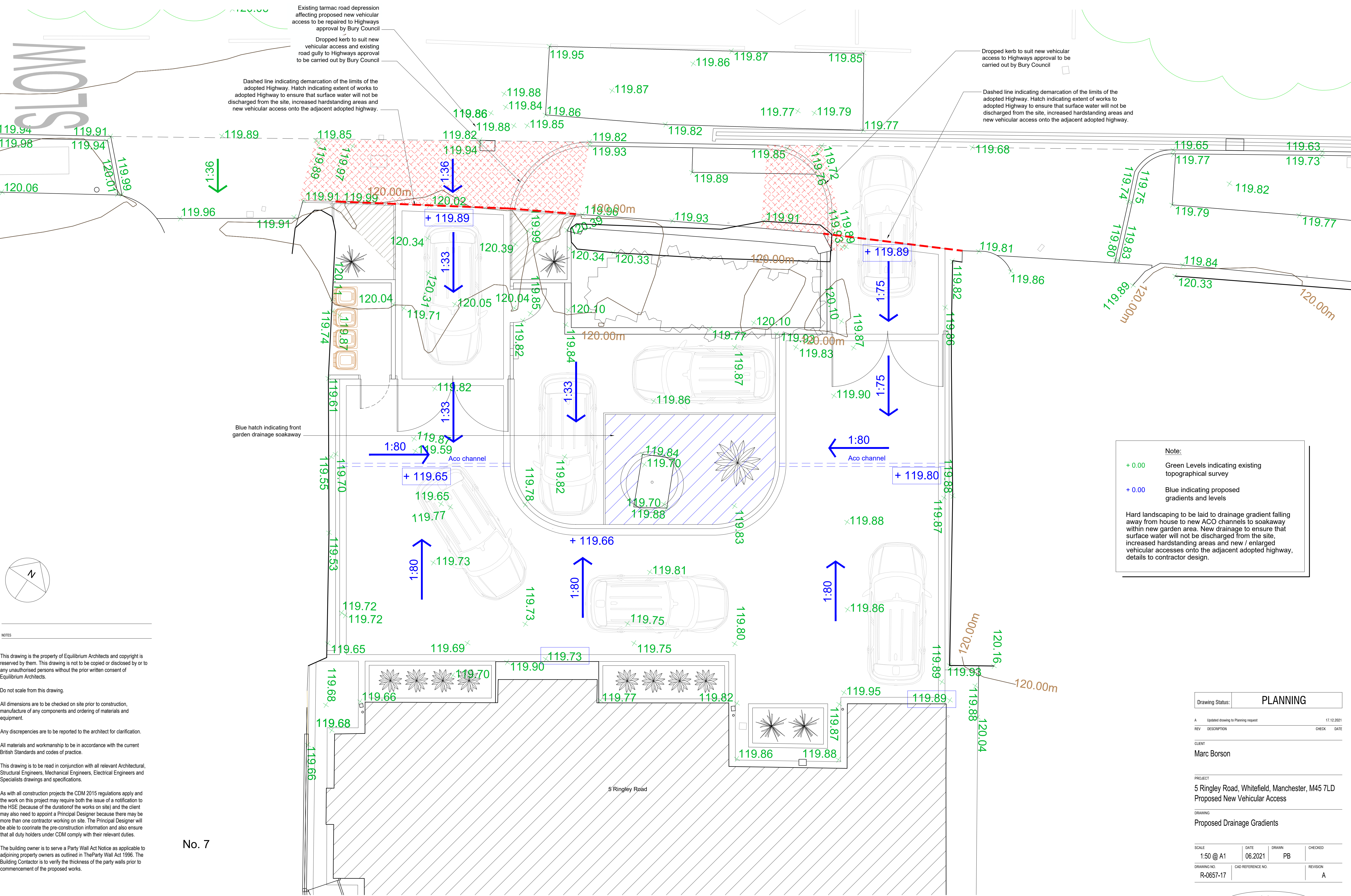
Proposed Drainage Gradients Scale 1:50
