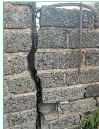
Large crack in the chicken coop wall
