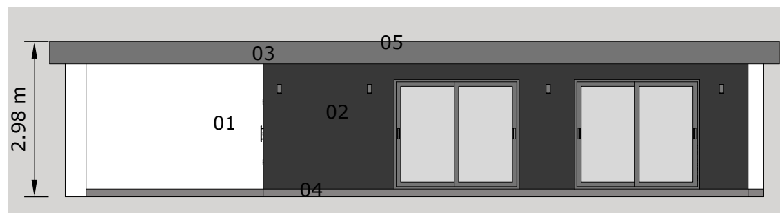
North Elevation
