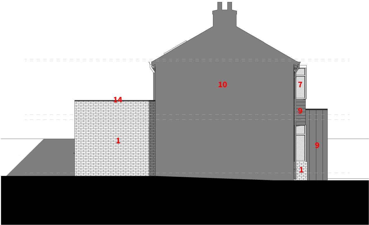
Proposed Party Wall Elevation 1:100 @ A3
