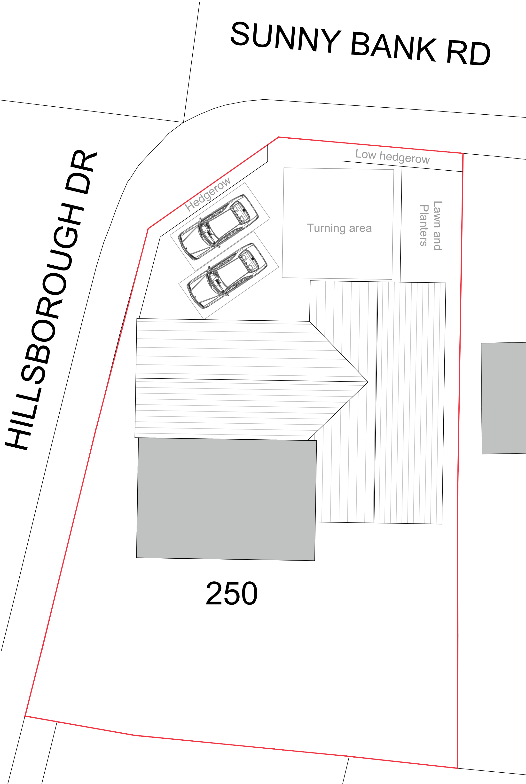
Proposed Roof and Block Plan 1:100 Scale @ A1
