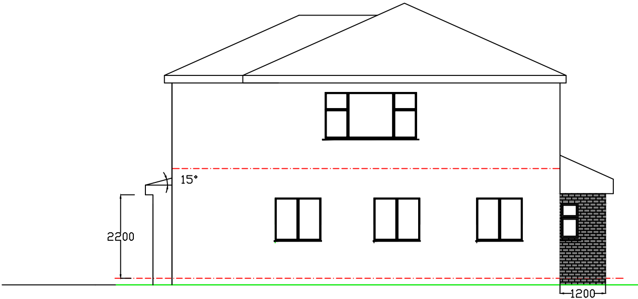
Side Elevation
