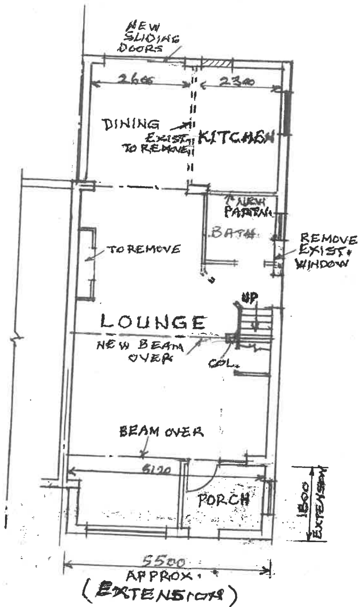
GROUND FLOOR (PROPOSED)
