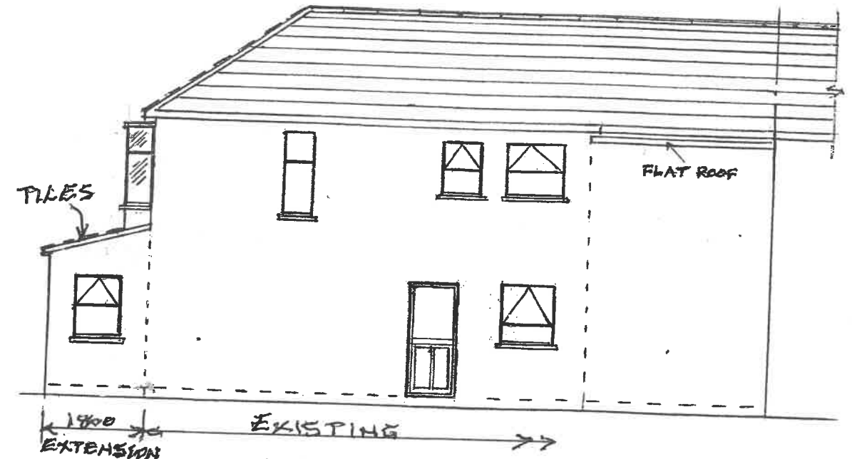
R.H.S. ELEVATION (PROPOSED)
