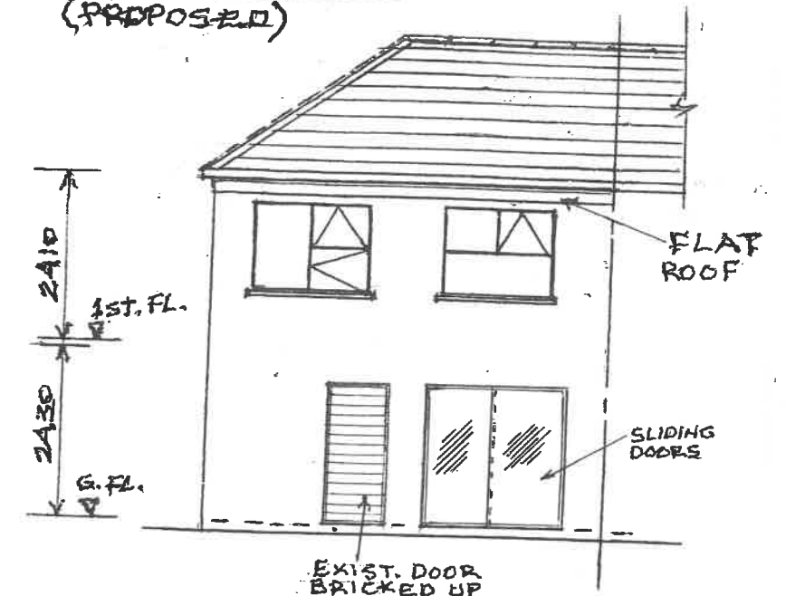
REAR ELEVATION
