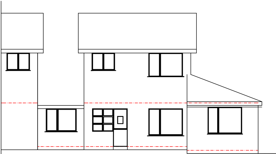
Rear Elevation
