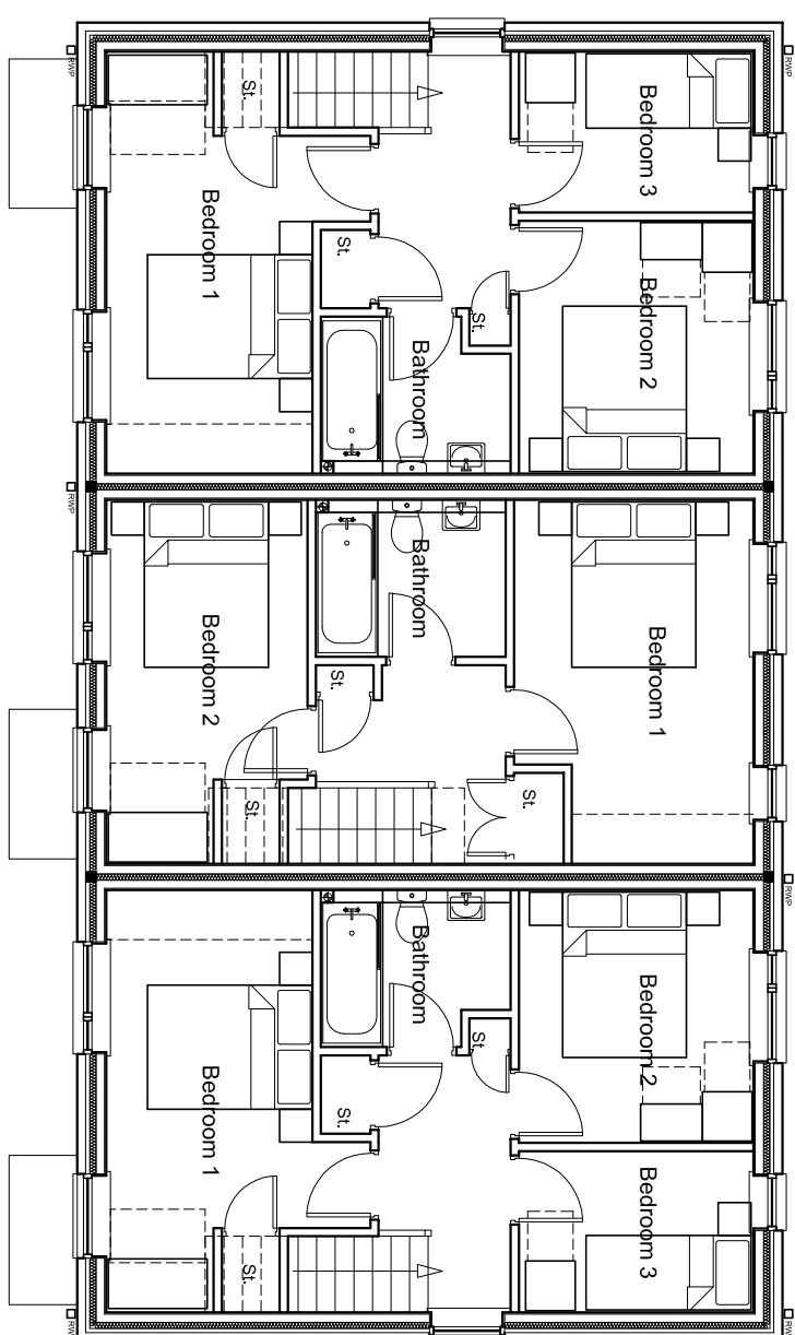
First Floor Plan Plot's 3 - 5
