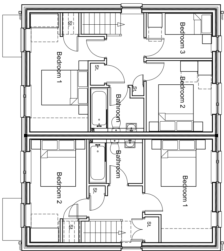
First Floor Plan Plot's 1 - 2 & 19 - 22
