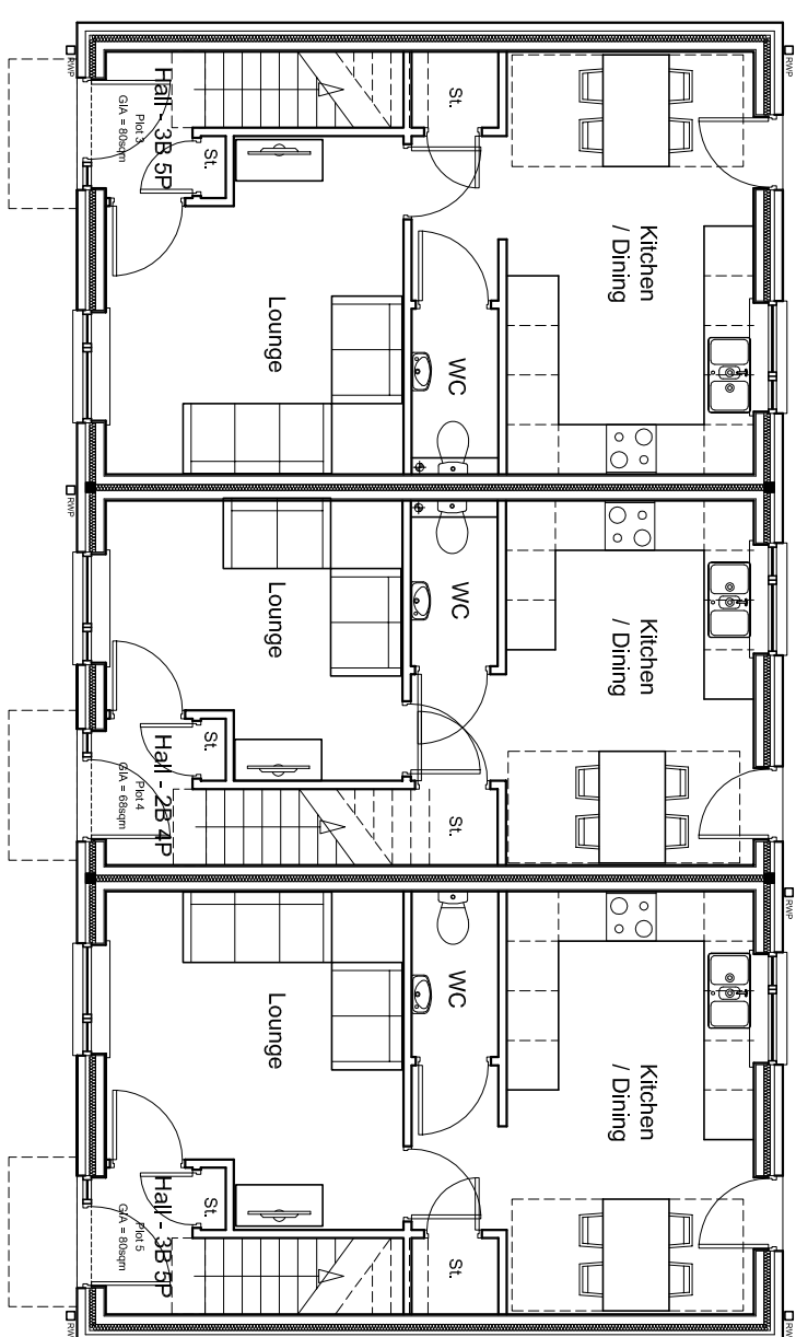
Ground Floor Plan Plot's 3 - 5
