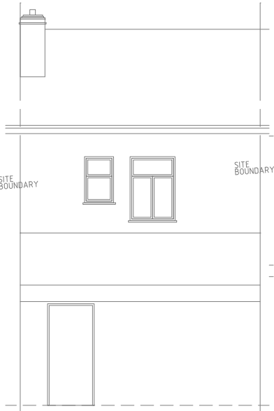
SIDE ELEVATION (EXISTING)
