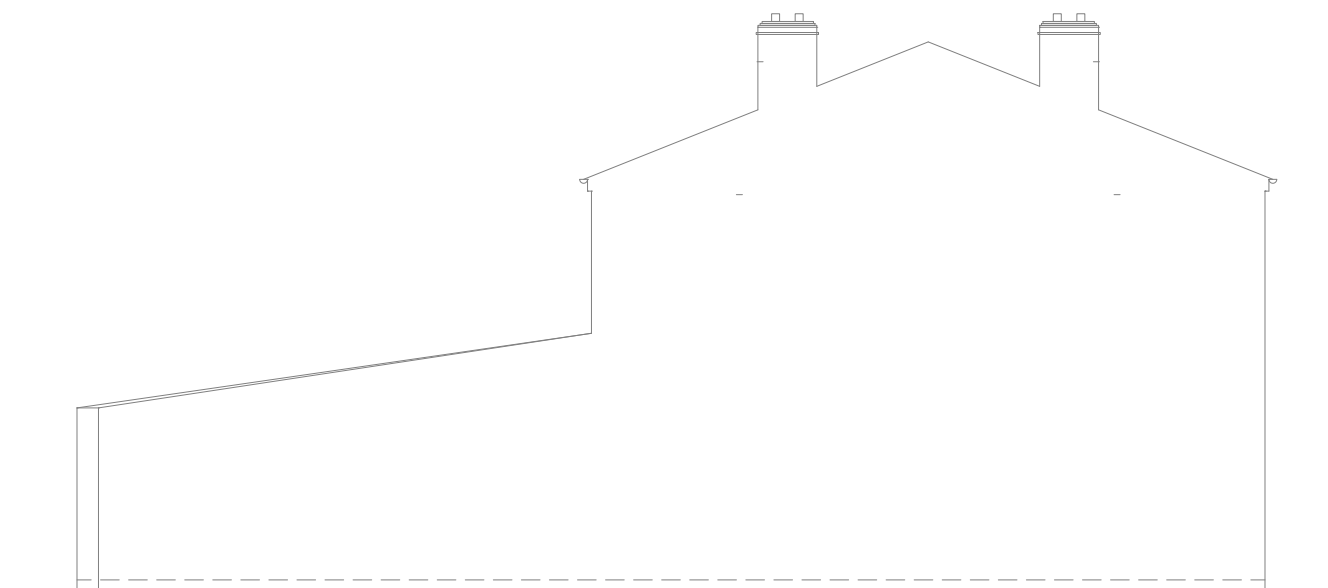
SIDE ELEVATION (EXISTING)
