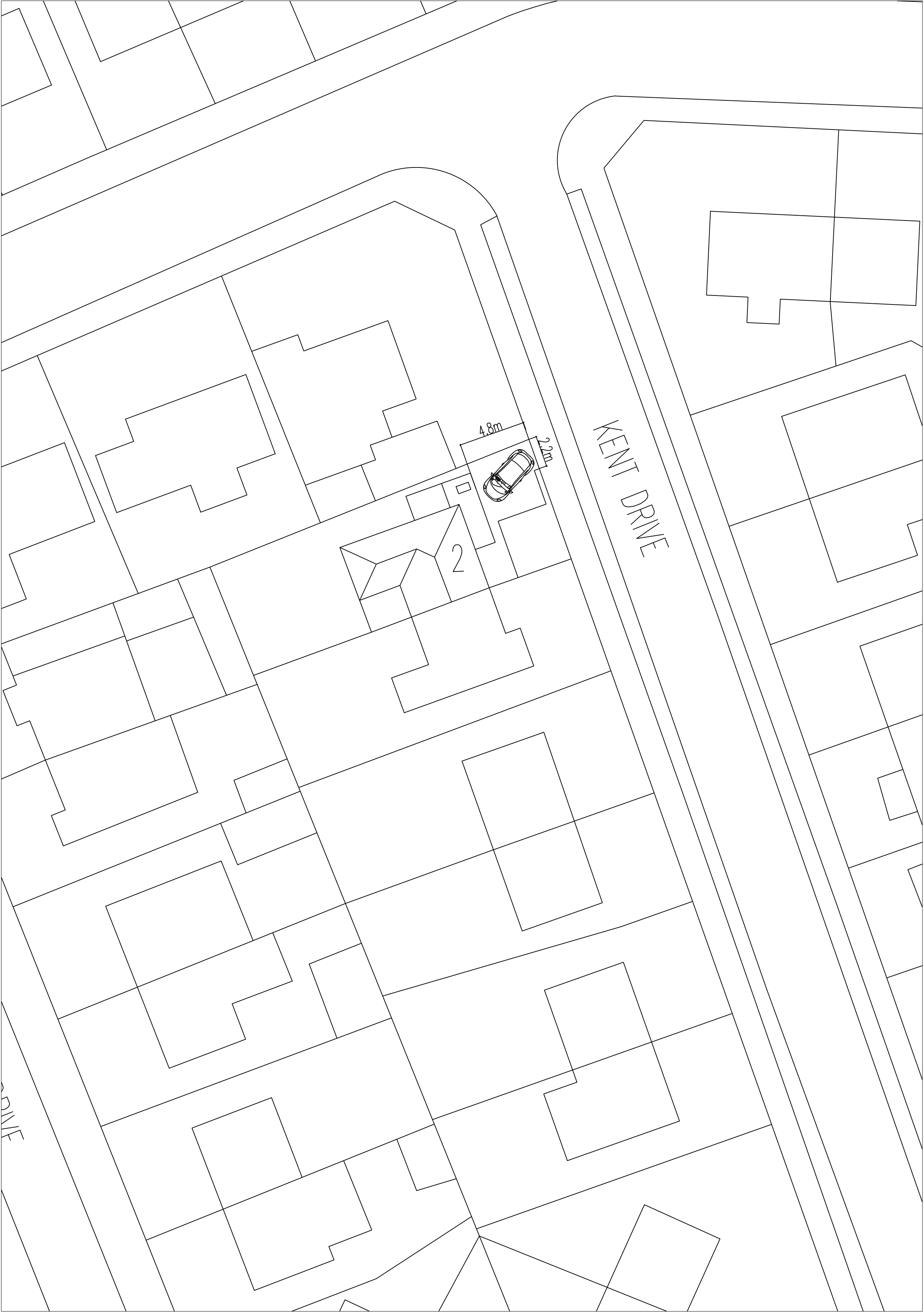
02 Proposed Parking Plan Scale 1:200
