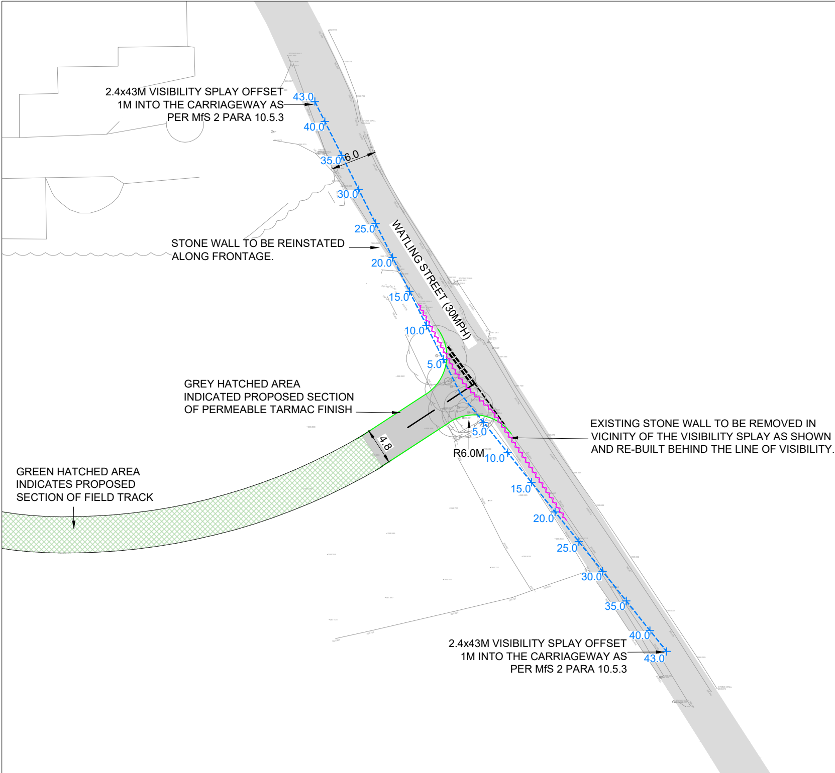
ADOPTED HIGHWAY PLAN
